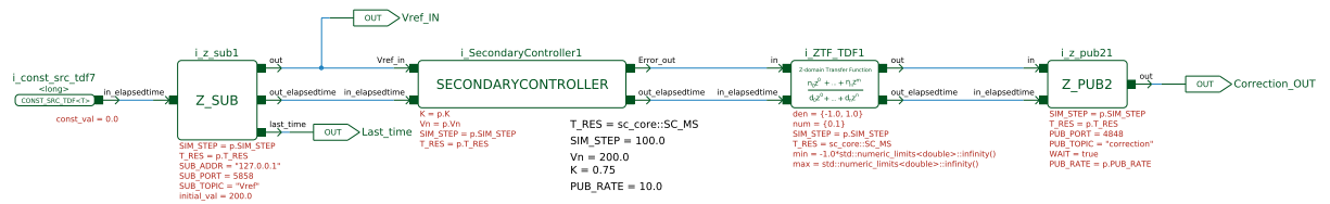
Figure 5: SystemC-AMS schematic of the secondary controller. The block following the relay block Z_SUB calculates the difference between the nominal voltage and the reference voltage, which is then multiplied by the secondary constant k_s . It is then integrated using a TDF block that implements integration as a z-transform. The publisher relay block Z_PUB2 receives the required correction from the integrator block, along with the cumulative time elapsed for the given simulation step, and adds wait time to the scheduler to induce real-time behavior.
