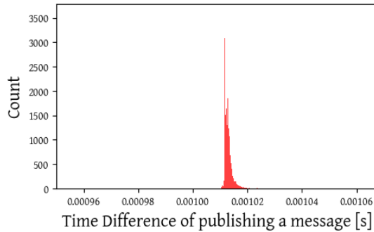
Figure 9: Histogram of time differences of publication time-stamp of timeliness of publication of messages.
